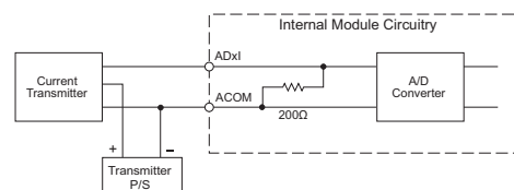
Analogue Current Input Circuit
