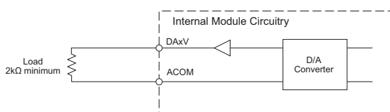
Analogue Voltage Output Circuit
