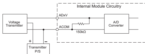
Analogue Voltage Input Circuit
