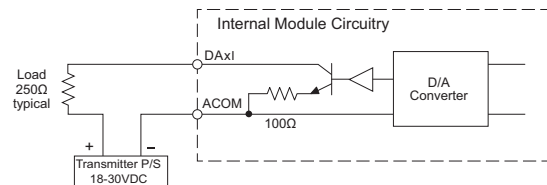
Analogue Current Output Circuit
